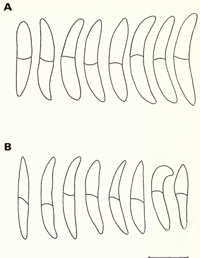
Fig. 21 Ascospore outlines of Leptorhaphis tremulae Körber (A) H-NYL 730-lectotype of Verrucaria sphenospora ; (B) L-lectotype & WRS�-isotype of Leptorhaphis tremulae ; scale = 10 µm.
